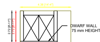
MAIN GATE ELEVATION
