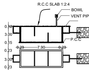
SEPTIC TANK AND TRENCH NTS
