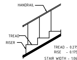
STAIRCASE DETAILS NTS
