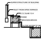
DETAILS OF FILTER BED & WELL NTS
