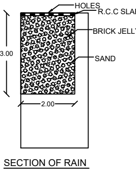
SECTION OF RAIN
