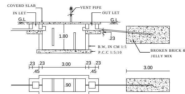
PLAN &amp; SECTION OF SEPTIC TANK &amp; TRENCH
