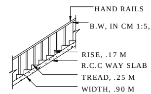
SECTION ON STAIR
