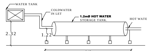
SOLAR WATER HEATING SWHS DETAIL
