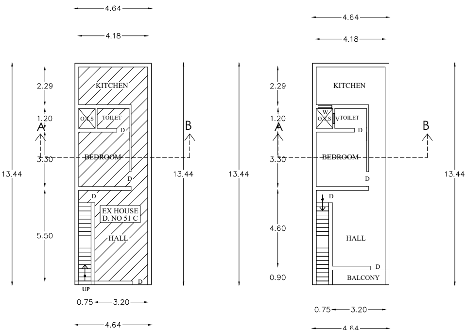
EX GROUND FLOOR PLAN
