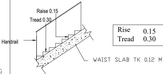
STAIRCASE DETAIL
