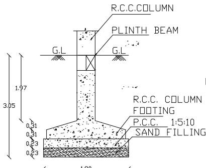
FOUNDATION DETAIL
