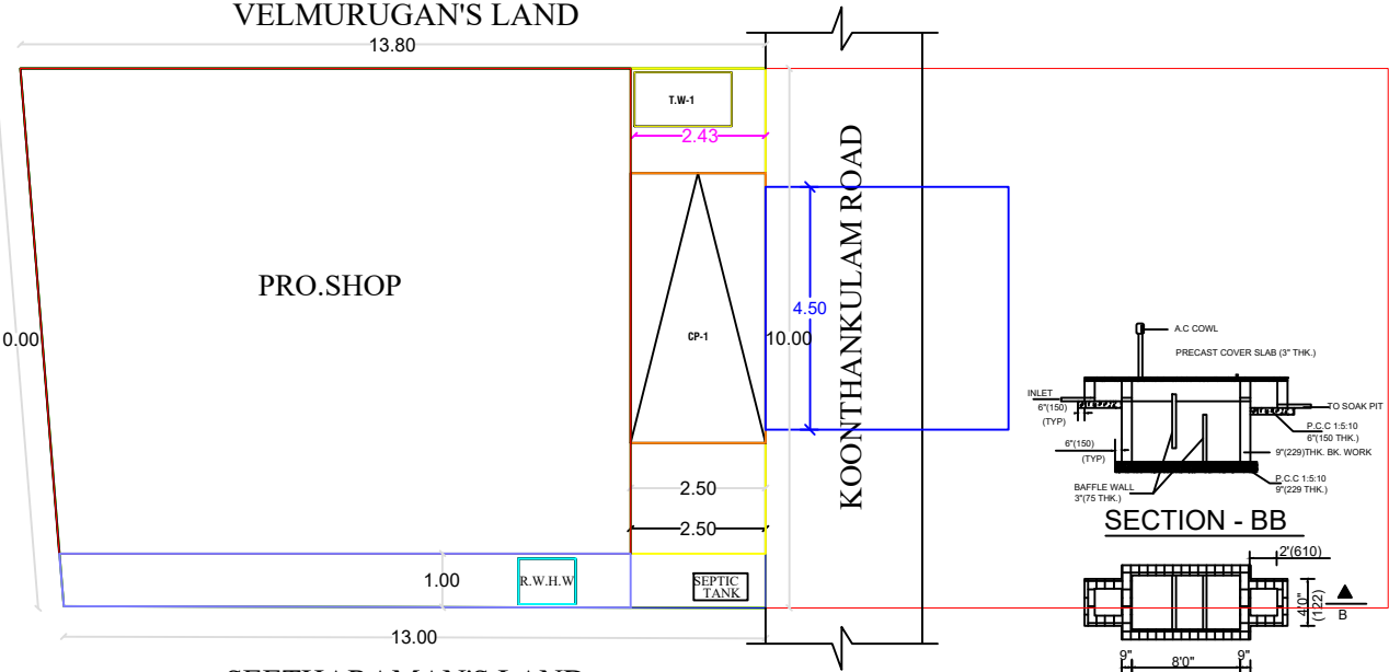
SEETHARAMAN'S LAND SITE PLAN
