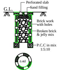
PERCOLATION PIT (NOT FOR SCALE)
