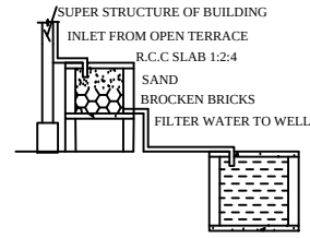
Rainwater harvesting
