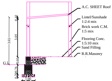
SECTION
