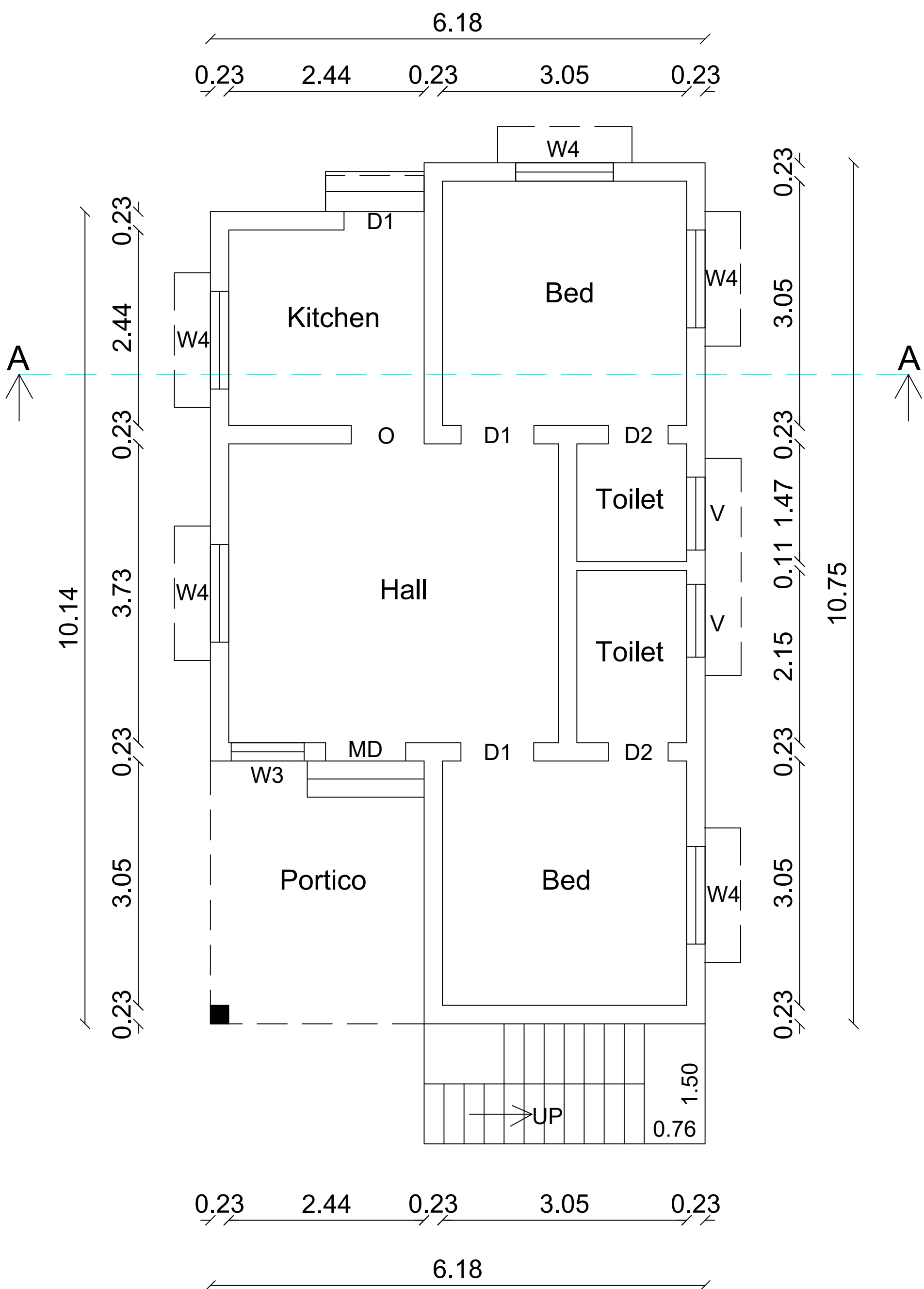
PLAN
