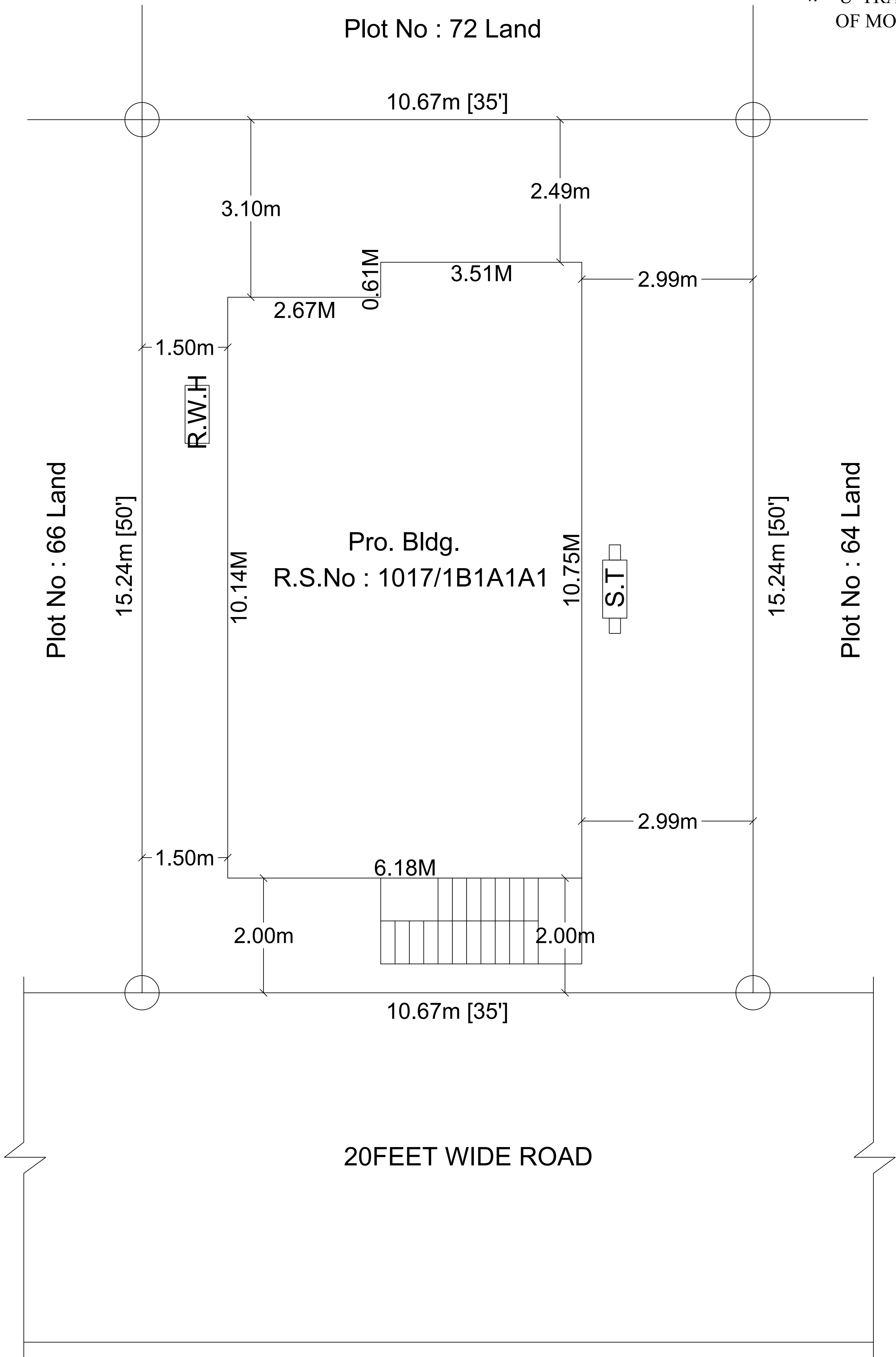
SITE PLAN
