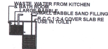
RECYCLING OF WASTE WATER FROM KITCHEN & BATHROOM
