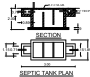
SEPTIC TANK PLAN
