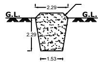
TRIAL PIT (Scale 1:100)
