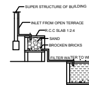
DETAILS OF FILTER BED & WELL NTS
