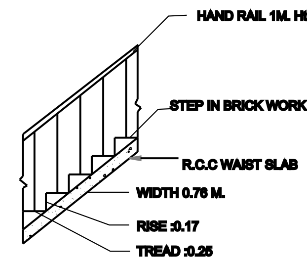
STAIR DETAIL
