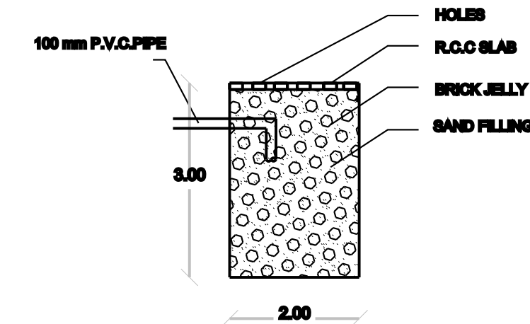
SECTION OF RAIN WATER COLLECTING TANK
