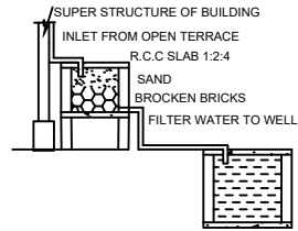
RAINWATER HARVESTING
