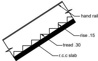
STAIR
