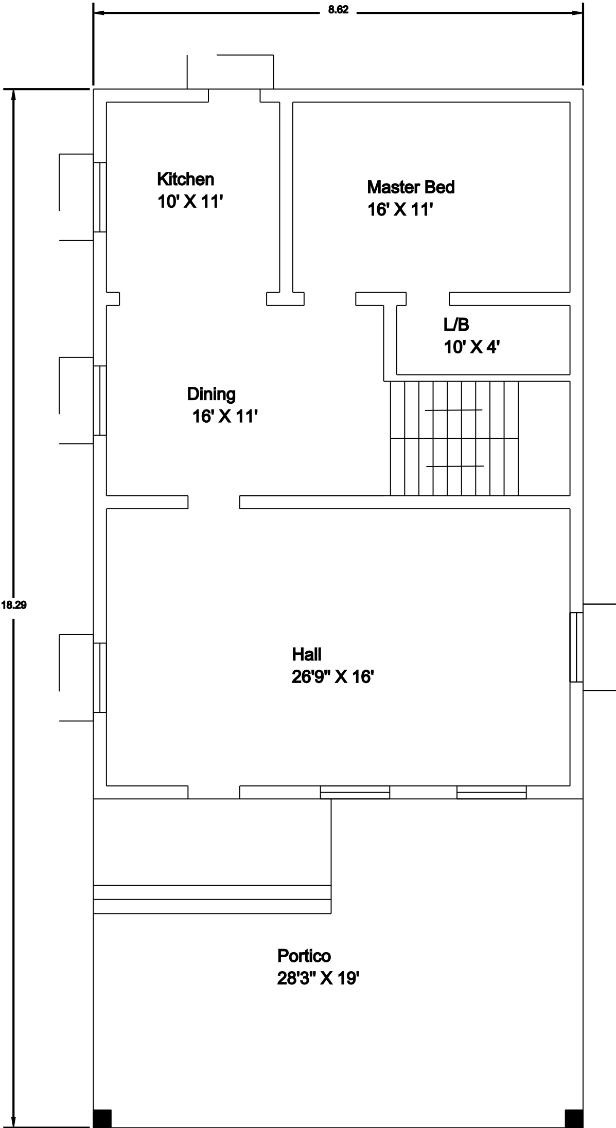
PLAN
