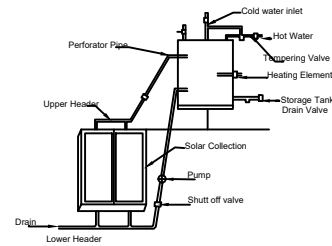
Details Of Solar Water Heater (NTS)
