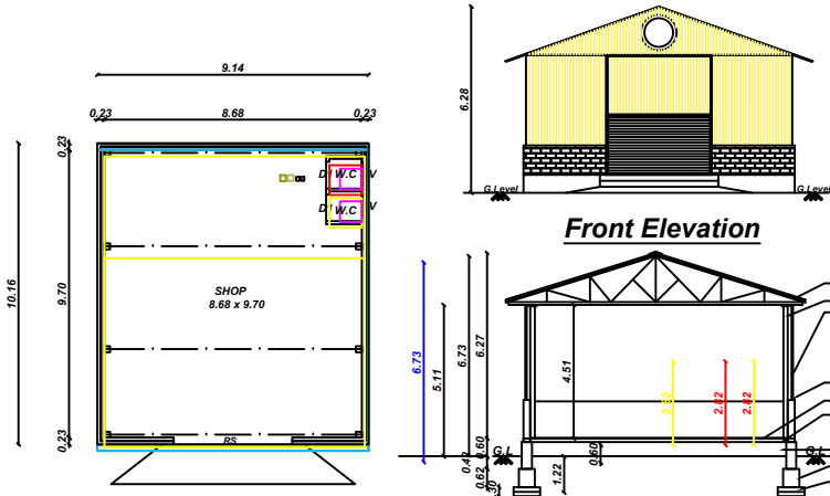
Ground Floor Plan (Proposed)
