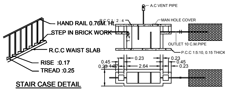
SEPTIC TANK DETAILS
