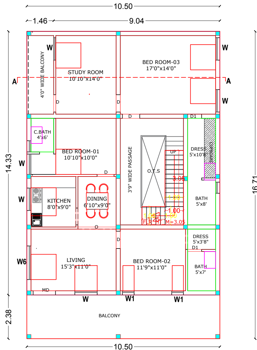
LAYOUT PLAN
