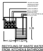
RECYCLING OF WASTE WATER FROM KITCHEN & BATHROOM
