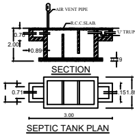
SEPTIC TANK PLAN
