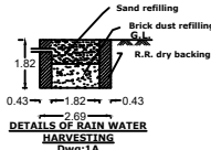
DETAILS OF RAIN WATER HARVESTING
