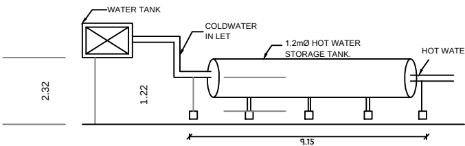
SOLAR WATER HEATING SWHS DETAIL
