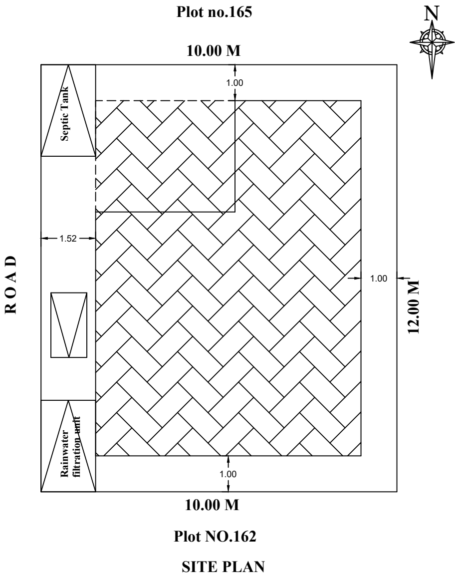
SITE PLAN
