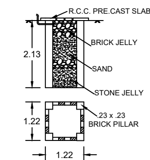
PLAN & SECTION OF RAIN WATER COLLECTION WELL
