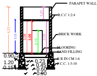
SECTION AB
