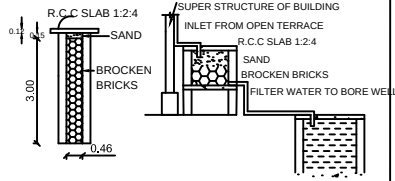
PERCOLATION PIT DETAILS OF FILTER BED & WELL
