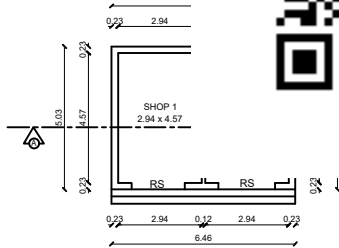
FLOOR PLAN
