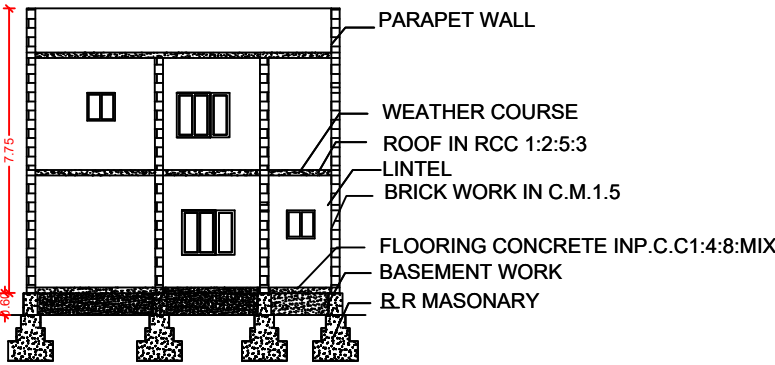
SECTION
