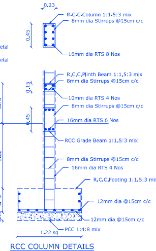
RCC COLUMN DETAILS
