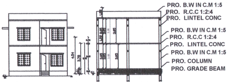
ELEVATION SECTION ON A A
