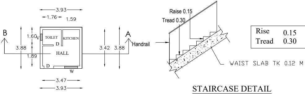
PRO GROUND FLOOR PLAN
