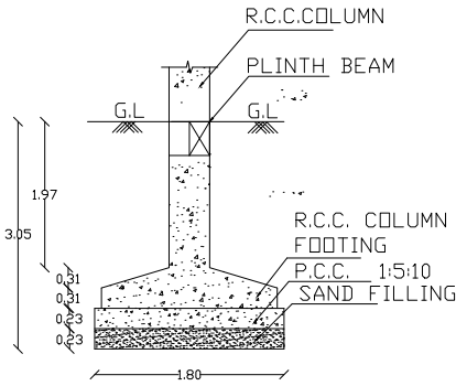
FOUNDATION DETAIL
