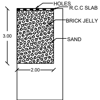
SECTION OF RAIN WATER COLLECTING TANK
