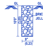
PERCOLATION PIT
