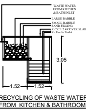
RECYCLING OF WASTE WATER FROM KITCHEN & BATHROOM (Scale 1:100)
