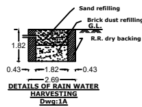
DETAILS OF RAIN WATER HARVESTING (Scale 1:100)
