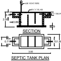
SEPTIC TANK PLAN (Scale 1:100)
