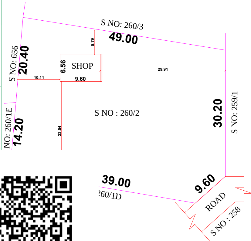
PLAN SCALE 1:200
