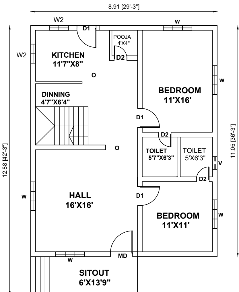
FLOOR PLAN
