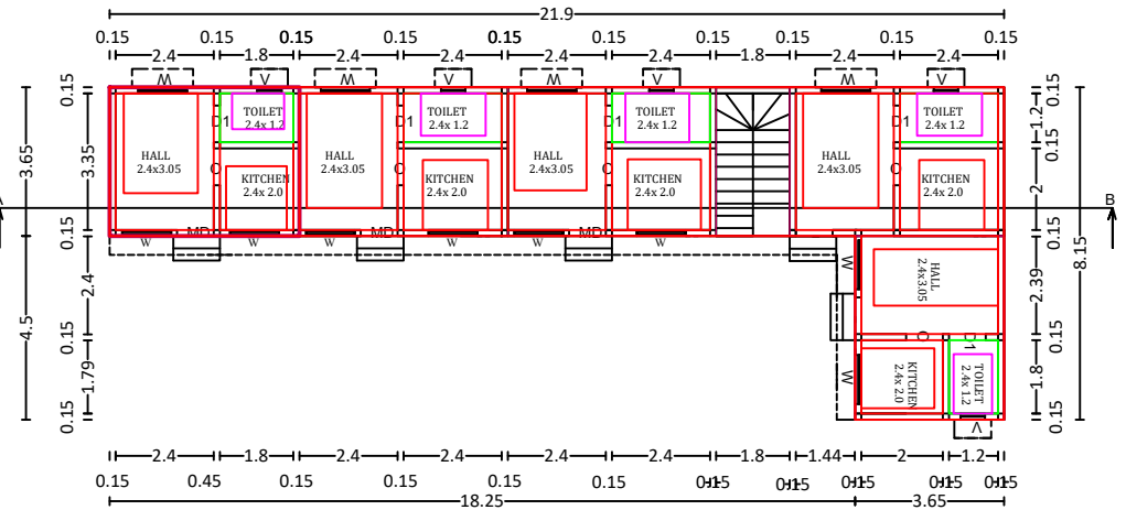
PLAN
