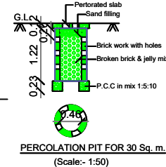
PERCOLATION PIT FOR 30 Sq. m. (Scale:- 1:50)
