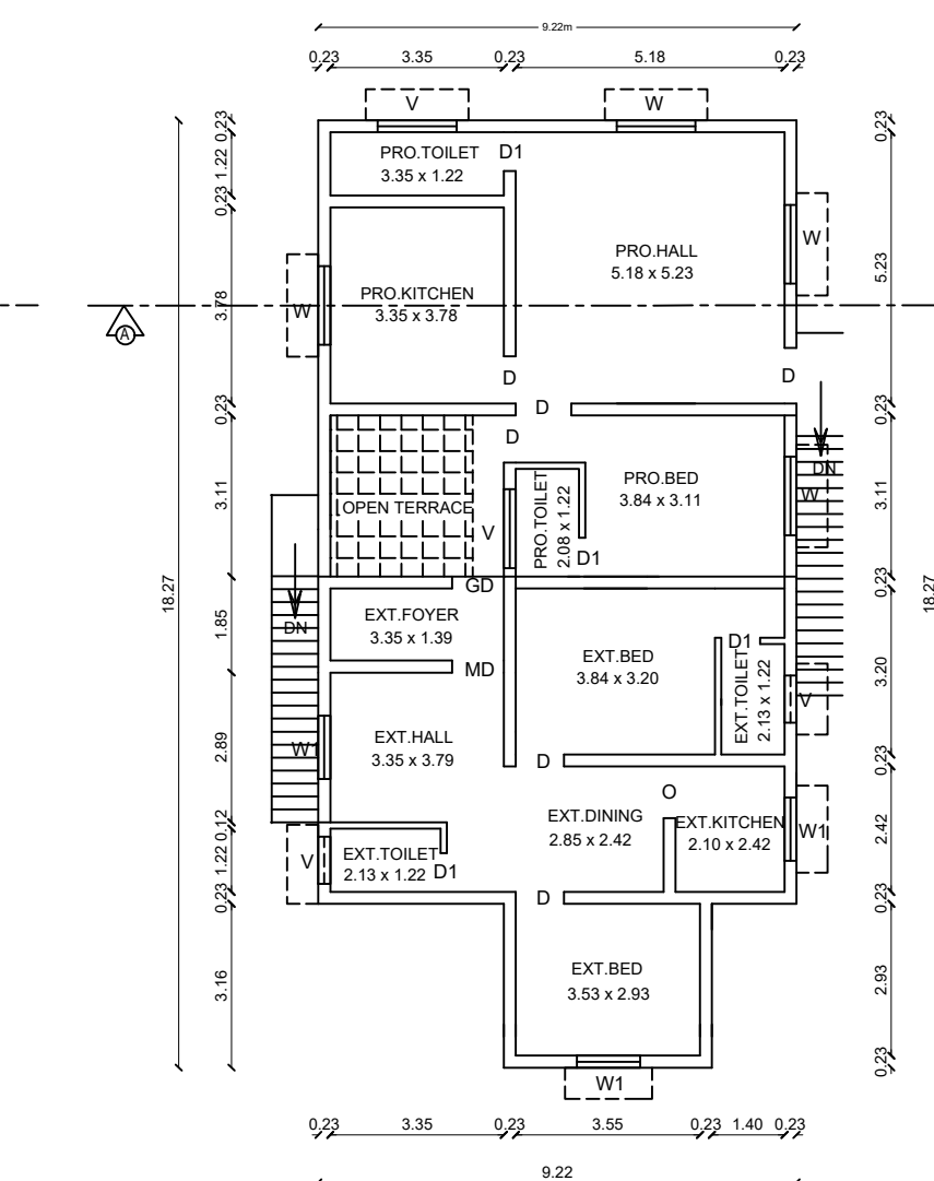
EXISTING AND PROPOSED FIRST FLOOR PLAN
