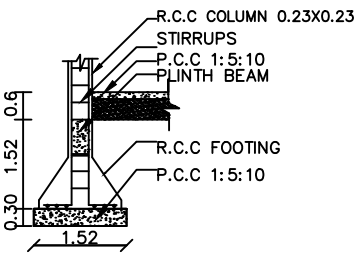
COLOUMN DETAILS
