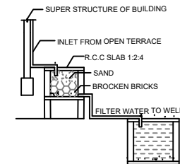
DETAILS OF FILTER BED & WELL NTS
