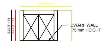
MAIN GATE ELEVATION
