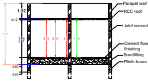
SECTION - "AB"
