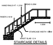
STAIRCASE DETAILS
