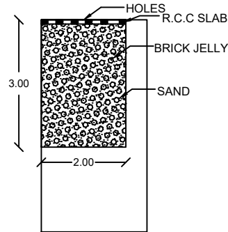
SECTION OF RAIN WATER COLLECTING TANK
