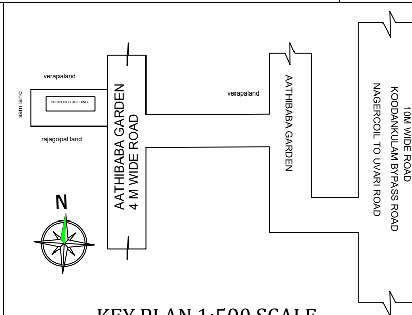
KEY PLAN 1:500 SCALE
