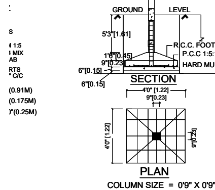
FOUNDATION DETAILS
