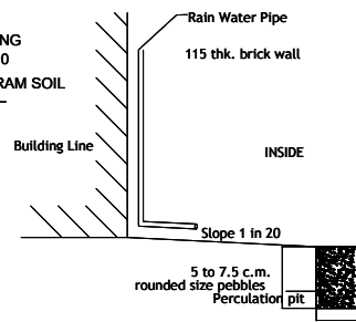
PERCOLATION PIT
