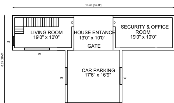
ALREADY APPROVED GROUND FLOOR PLAN
