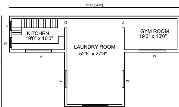
ALREADY APPROVED SECOND FLOOR PLAN
