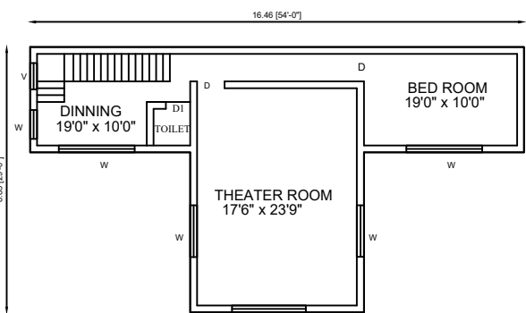
ALREADY APPROVED FIRST FLOOR PLAN
