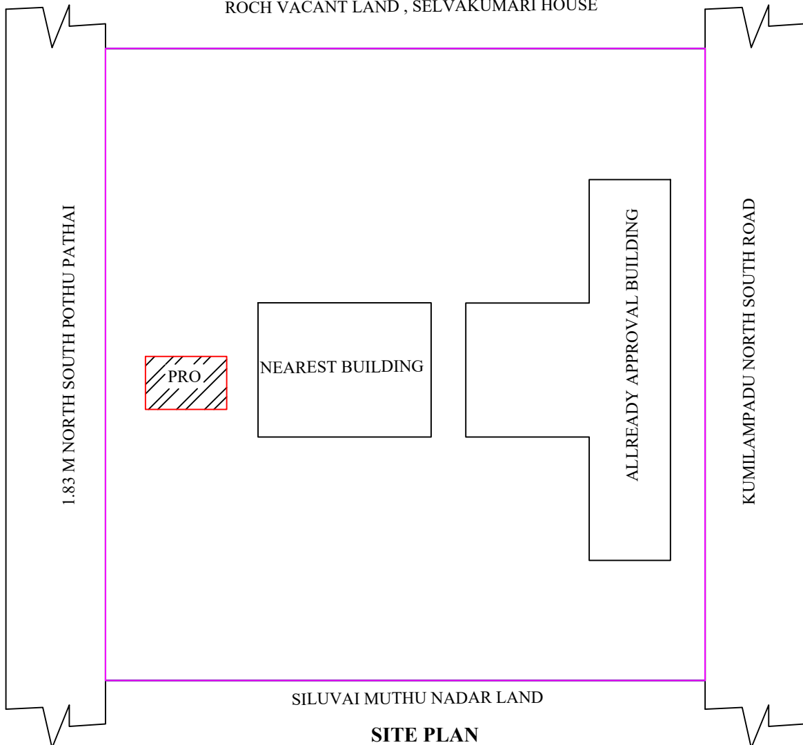
SITE PLAN
