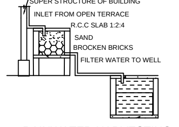
RAINWATER HARVESTING
