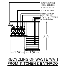
RECYCLING OF WASTE WATER FROM KITCHEN & BATHROOM
