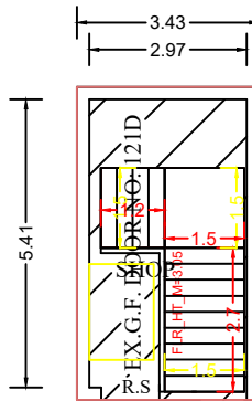
EX.G.FLOOR PLAN
