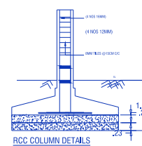
RCC COLUMN DETAILS
