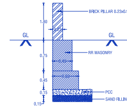
FOOTING DETAILS
