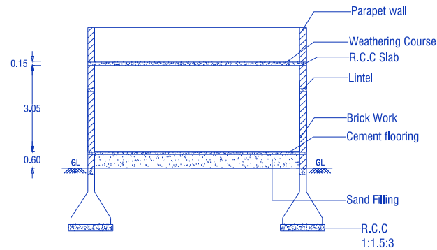
CROSS SECTION ON 'AB'
