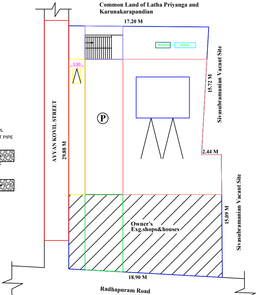
SITE PLAN
