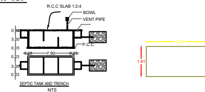
SEPTIC TANK AND TRENCH NTS
