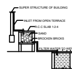
DETAILS OF FILTER BED & WELL NTS
