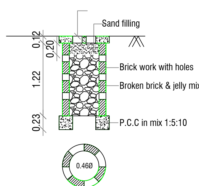
PERCOLATION PIT FOR 30 Sq. m.
