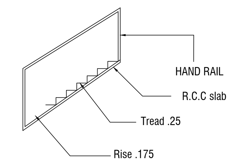
STAIR DETAIL
