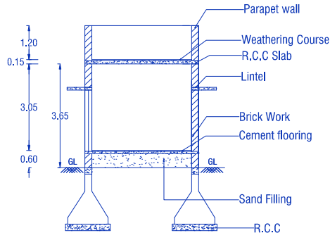
CROSS SECTION ON 'AB'
