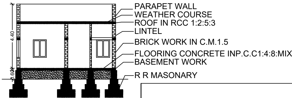
SECTION
